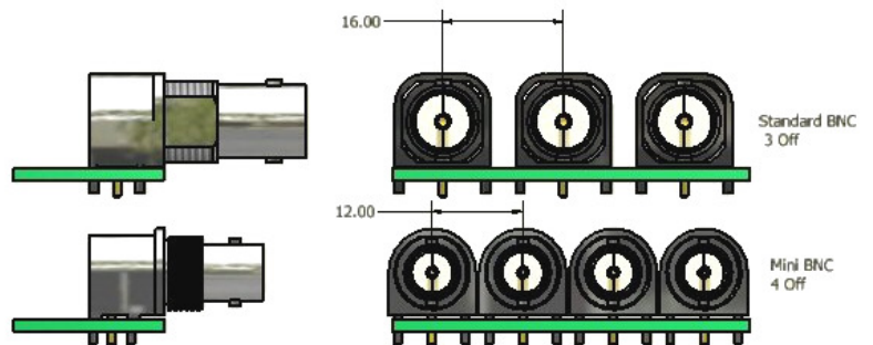
Pitch comparison between Standard BNC and Mini BNC Connectors
